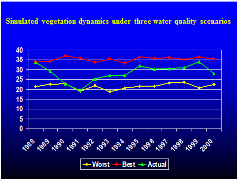
Figure 1. Percent occurrence of SAV in Pool 8 under three different water turbidity scenarios (observed best, worst and annual actual).
